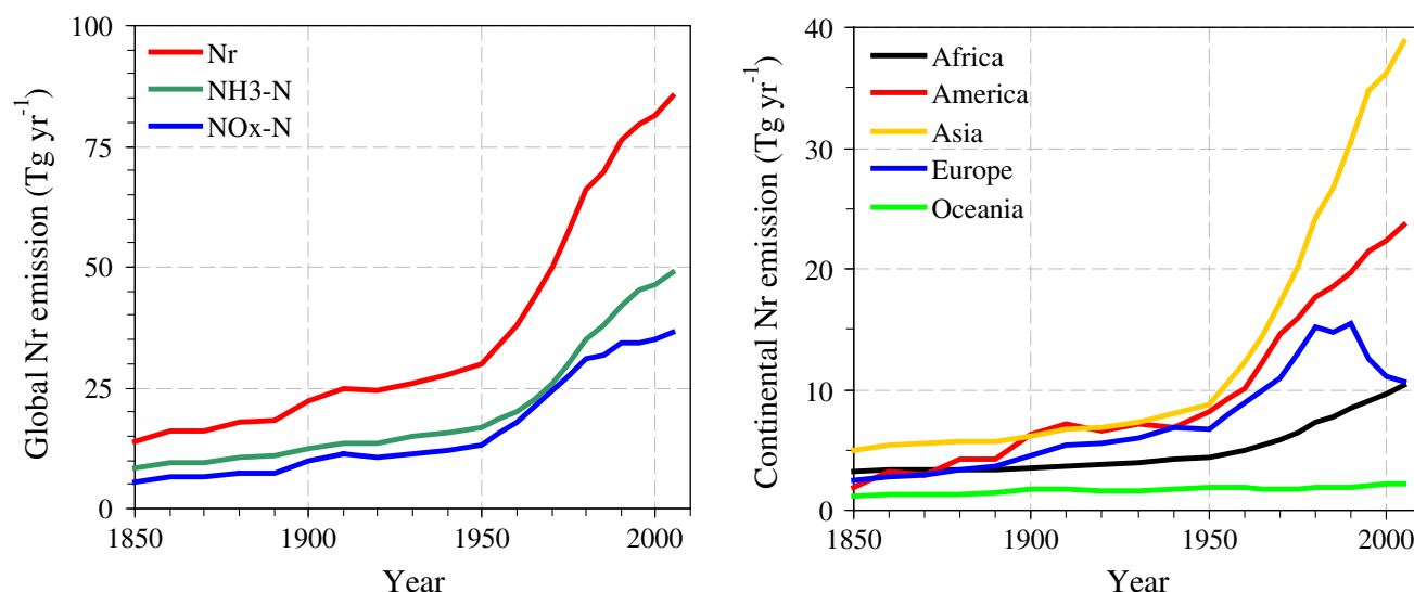
Fig. 2 Global (left panel) and continental (right panel) annual rates of Nr (NO x -N + NH 3 -N) emissions (derived from Kopáček and Posch 2011)
